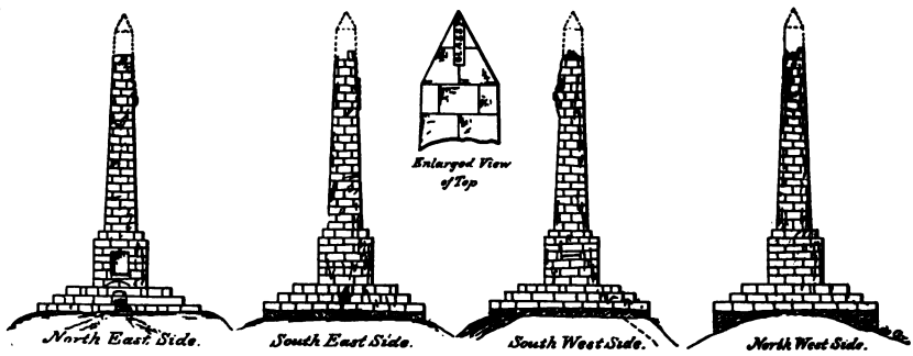
Fig. 3. Sutherland Monument, struck April 28, 1884. From Jour. Met. Soc., Walker.
